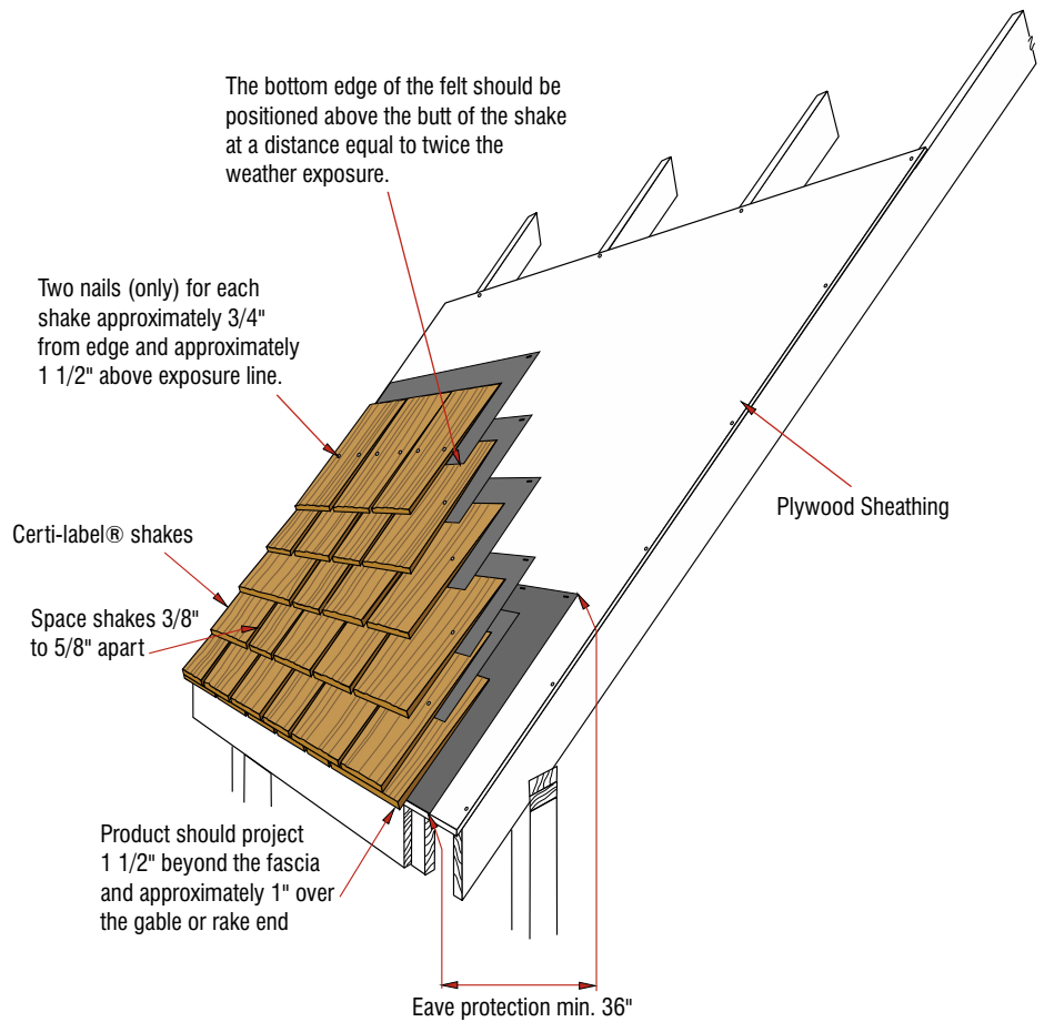
Figure 6: Mansard Roof
