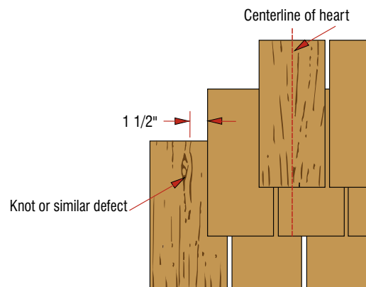
Figure 5a: Course Alignment
