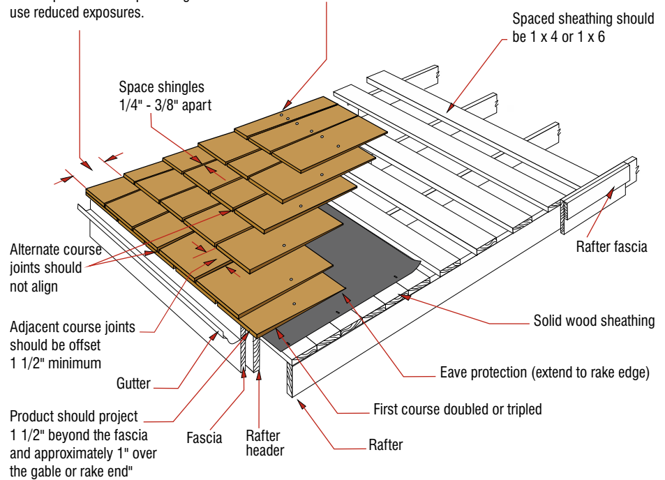
Figure 5: Certi-label® Shingle Application
