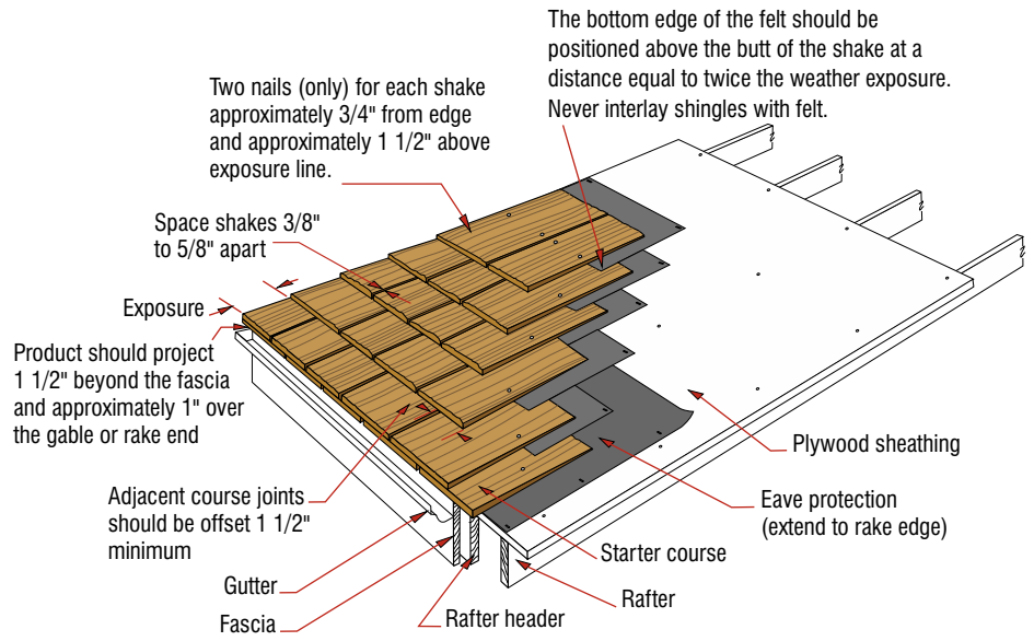
Figure 21a: Certi-Last® Shake Application (Option 1 Depicted)
