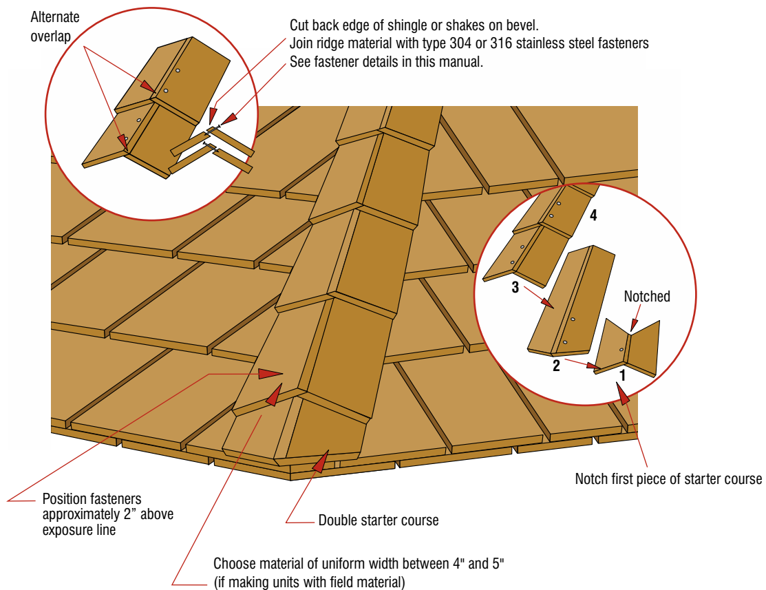
Figure 8: Certi-label® Hip and Ridge Application
